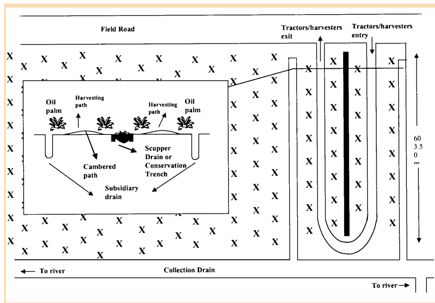
Figure 1. Field layout for flat land zero burning oil palm replanting.
